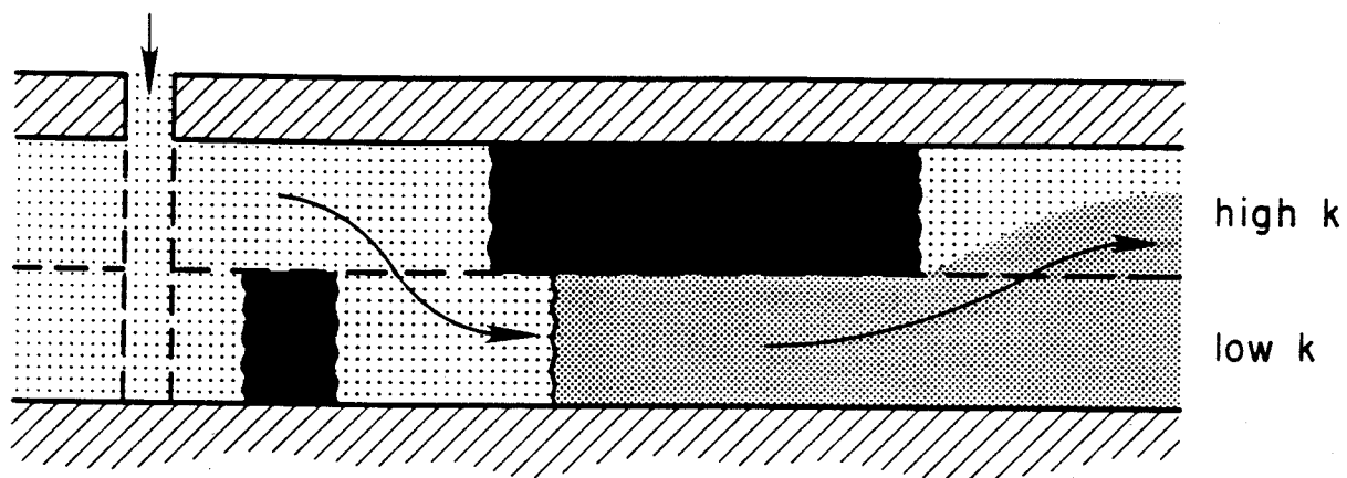
(a) Poor Sweep Prior to Gel Treatment — Treatment is Effective
