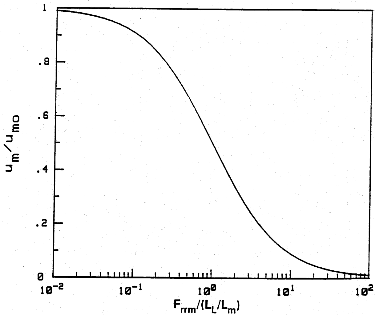
Fig. 22. Effects of F_{rrm} and L_L/L_m on flow in the rock matrix.
