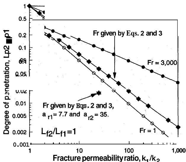
Fig. 8—Degree of penetration vs. fracture permeability ratio.
