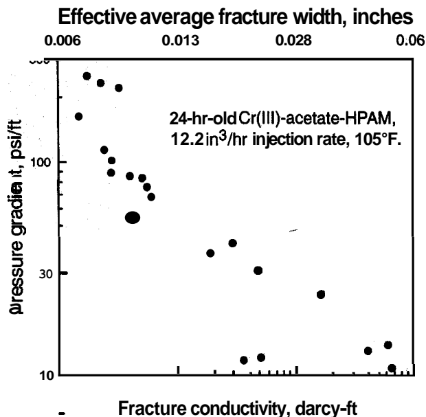
Fig. 2—Pressure gradient vs. fracture conductivity and width.
