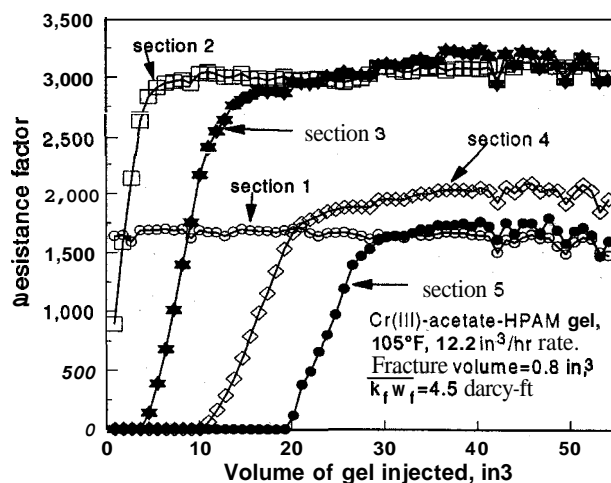
Fig. 5—Resistance factor vs. volume of gel injected in a fractured core (3.8-ft long).
