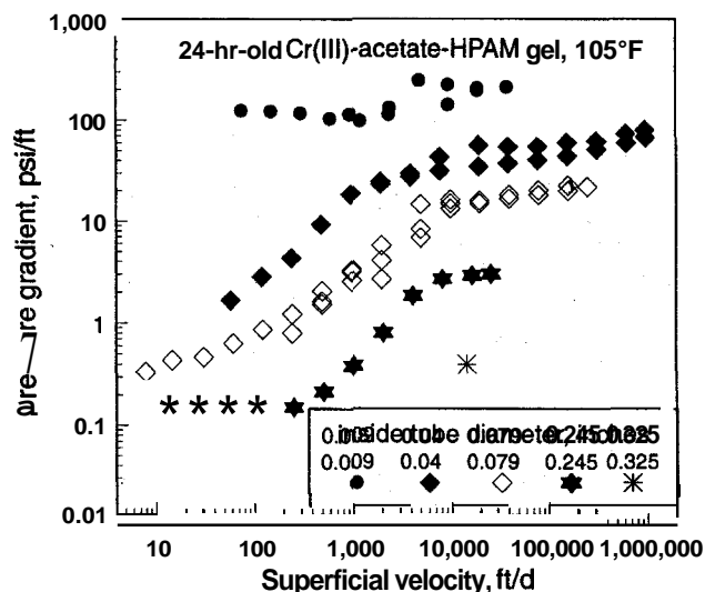
Fig. 4—Pressure gradient vs. velocity for gel in tubes.
