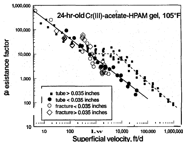
Fig. 3—Comparison of resistance factors in fractures vs. in tubes.
