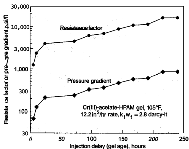
Fig. 7—Effect of gel age on resistance factors and pressure gradients in a fracture.
