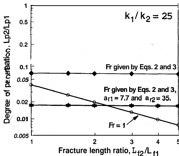
Fig. 9—Degree of penetration vs. fracture length ratio.
