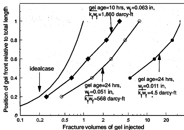
Fig. 6—Gel propagation through fractures (3.8–4.0 ft long).
