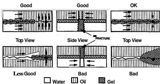
Fig. 1—Idealized placement locations for gels in fractures.
