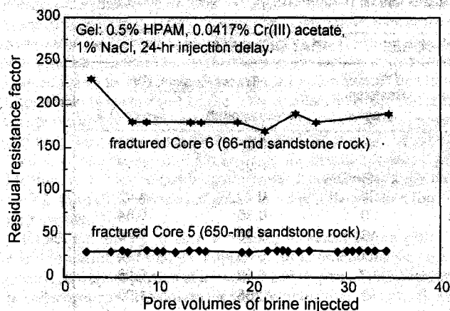
Fig. 10—Residual resistance factor vs. throughput after gel placement.
