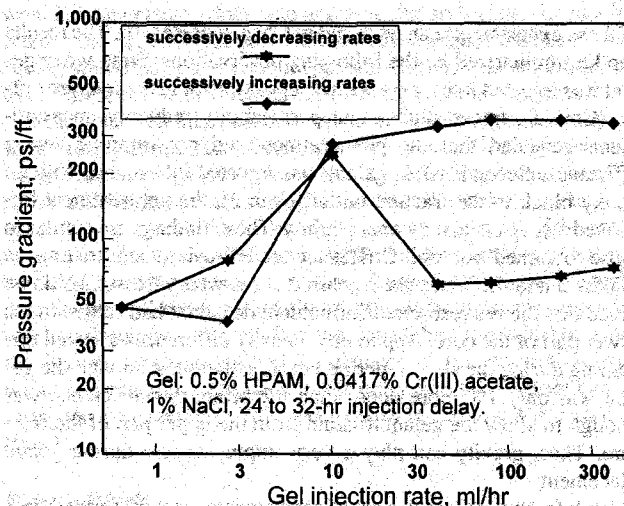
Fig. 9—Pressure gradient during placement of a Cr(III)/acetate/HPAM gel.
