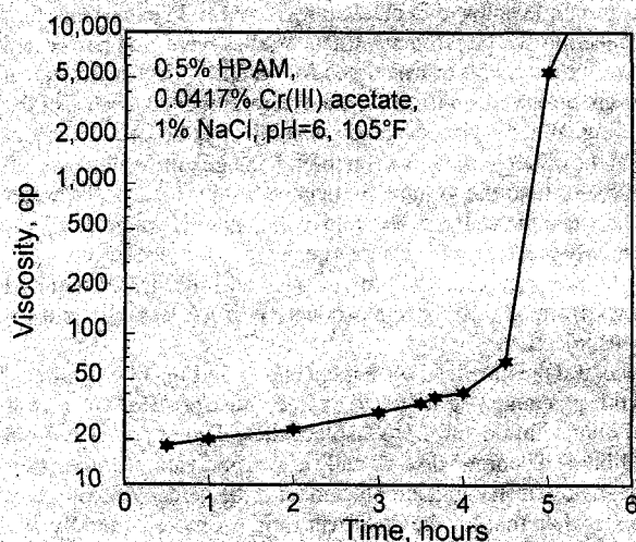
Fig. 2—Viscosity vs. time during gelation.
