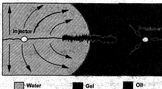
Fig. 1—Idealized gel placement in fractured wells.
