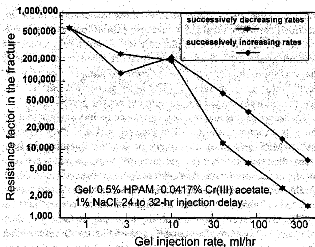
Fig. 8—Resistance factor in the fracture during placement of a Cr(III)/acetate/HPAM gel.
