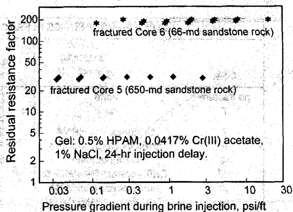
Fig. 11—Residual resistance factor vs. pressure gradient after gel placement.
