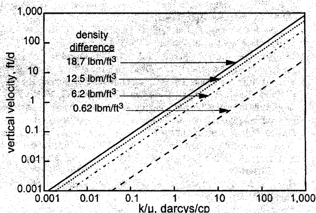
Fig. 12—Vertical velocity vs. k/\mu and density difference.
