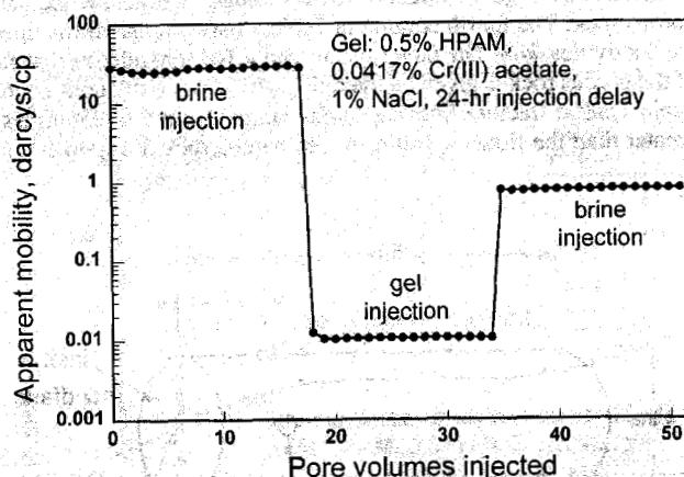
Fig. 7—Effect of brine and gel throughput on apparent mobility in fractured Core 7.
