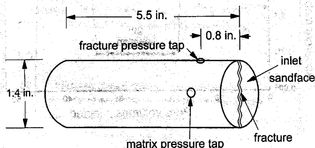
Fig. 4—Schematic of a fractured core.
