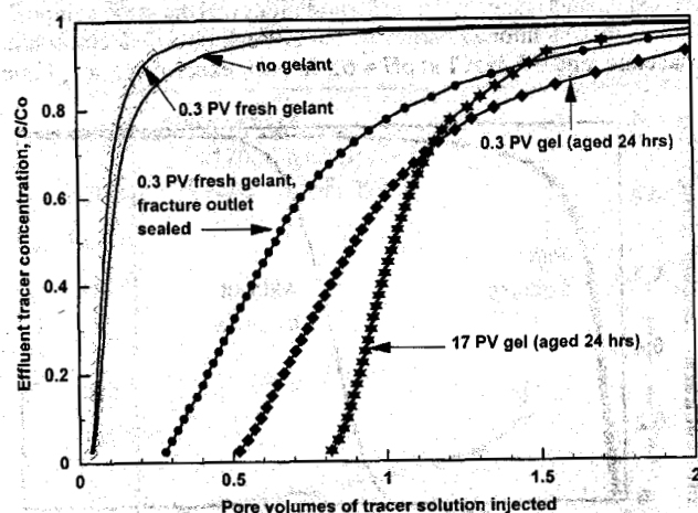
Fig. 6—Tracer results during brine injection after placement of Cr(III)/acetate/HPAM gelants or gels in fractured Berea sandstone cores.
