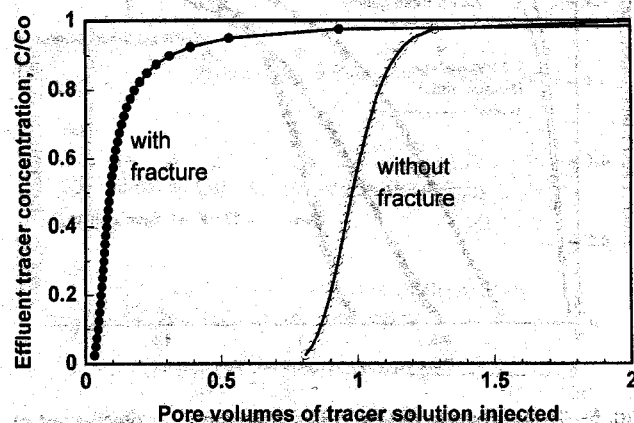
Fig. 5—Tracer results in fractured vs. unfractured Berea sandstone cores.
