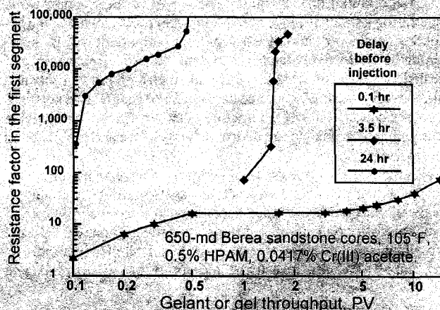
Fig. 3—Plugging in the first core segment for different delay times between gelant mixing and gelant injection.
